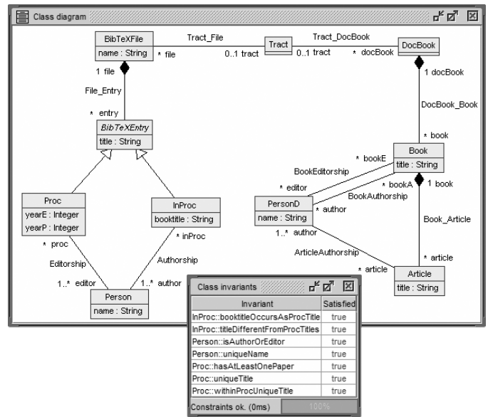
Fig. 7. Source and target metamodels.
