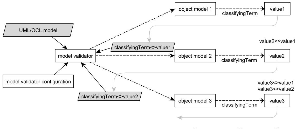
Fig. 4. Interplay between model validator and classifying term.
