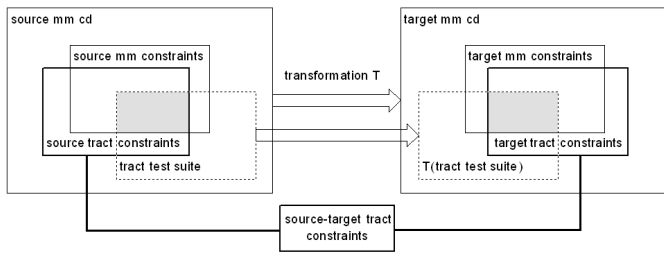
Fig. 6. Building blocks of a tract as in [3].
